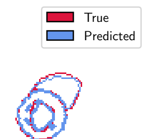
segmentations
